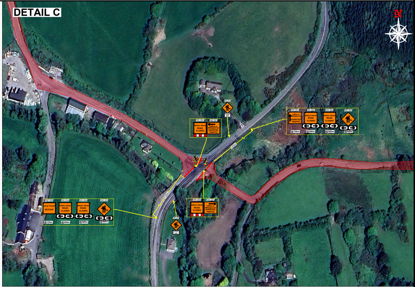
DETAIL C (WHEN CYCLIST ARE PASSING)
